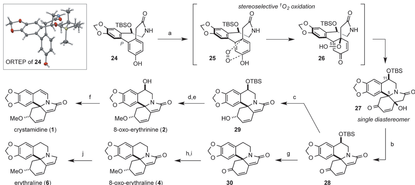
Scheme 3. Synthesis of the common intermediate and total syntheses of four erythrina alkaloids. Reagents and conditions: a) O 2 , hν , rose bengal, PPh 3 , NaHCO 3 , CH 3 CN/H 2 O (1:1), RT, 77%; b) SOCl 2 , pyridine, 0°C, 84%; c) NaBH 4 , CeCl 3 ·7H 2 O, CH 3 OH, RT, 75%; d) CH 3 I, NaH, THF, RT; e) TBAF, THF, RT, 84% (2 steps); f) TsOH·H 2 O (20 mol%), toluene, reflux, 77%; g) Et 3 SiH, BF 3 ·OEt 2 , CH 2 Cl 2 , 0°C, 74%; h) NaBH 4 , CeCl 3 ·7H 2 O, CH 3 OH, RT; i) CH 3 I, KOH, Et 4 NBr, THF, RT, 86% (2 steps); j) LiAlH 4 , AlCl 3 , THF/Et 2 O (1:1), 0°C, 73%.
